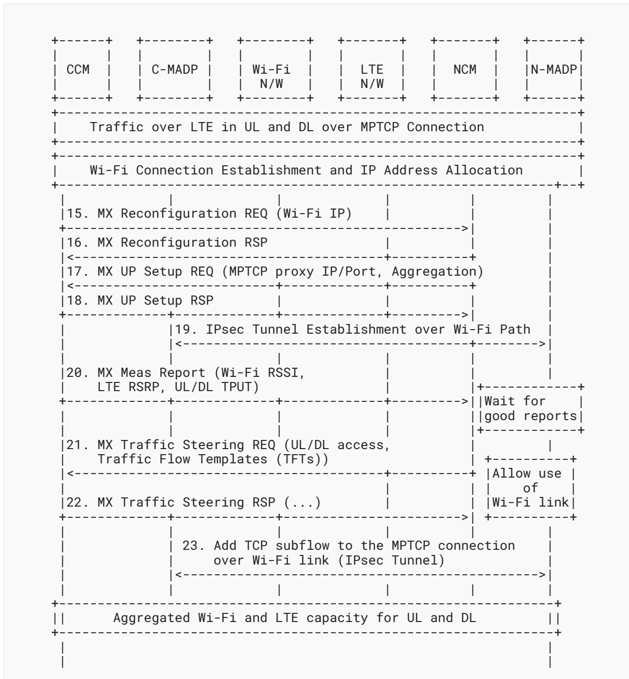
Figure 19: MAMS-Assisted MPTCP Proxy as User Plane - Add Wi-Fi Leg
